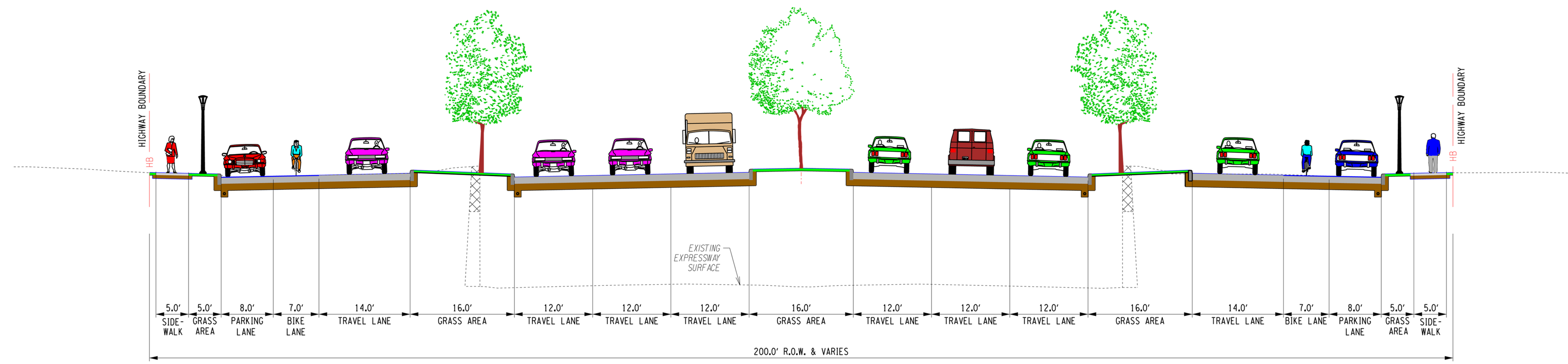
CONCEPTUAL TYPICAL SECTION BOULEVARD SECTION A-A
